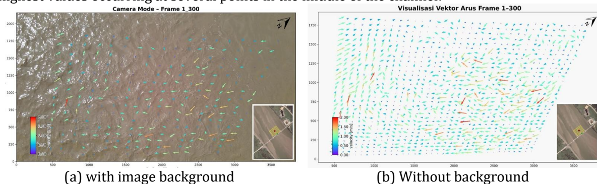
Figure 4. LSPIV analysis of surface-current vectors and velocities during the ebb phase
