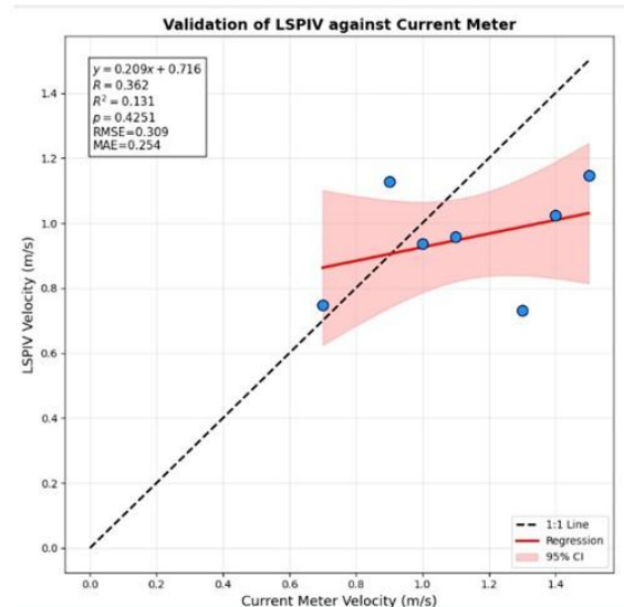
Figure 8. Validation of LSPIV against the current meter during the flood phase
