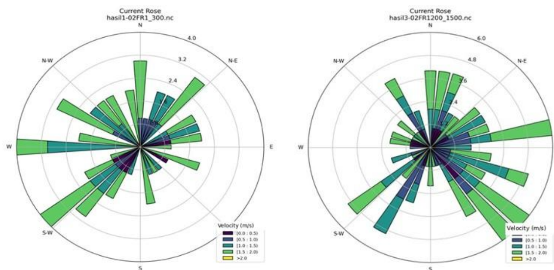
Figure 6. Current rose during the ebb phase (left) and flood phase (right)
