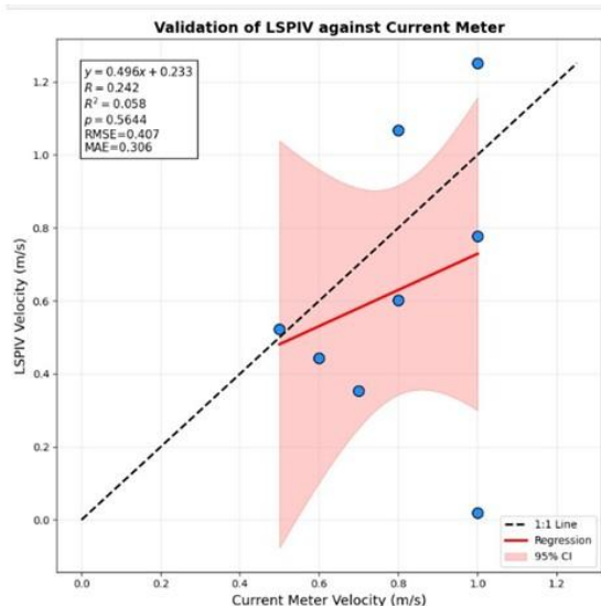
Figure 7. Validation of LSPIV against the current meter during the ebb phase
