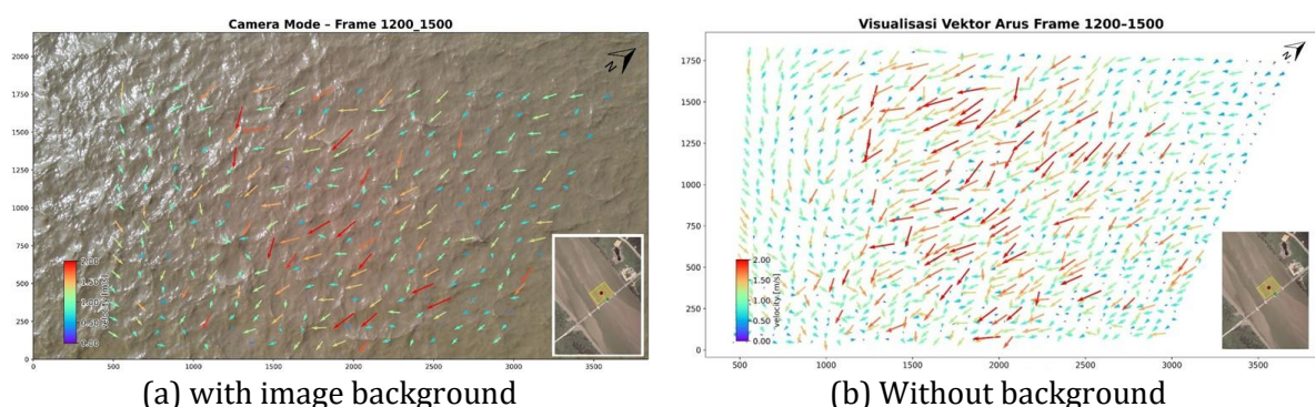
Figure 5. LSPIV analysis of surface-current vectors and velocities during the flood phase
